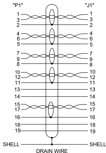
P1 DISPLAYPORT 2.0 MALE CONNECTOR
